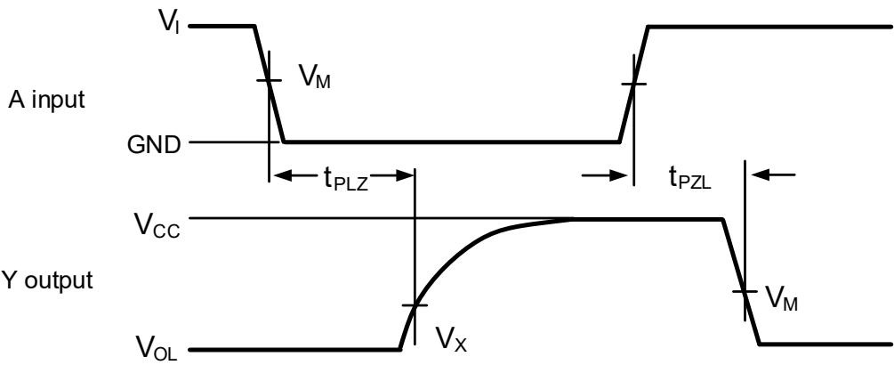
Figure 8-5 The data input (A) to output (Y) propagation delay times
