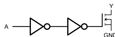
Figure 8-3 Logic diagram
