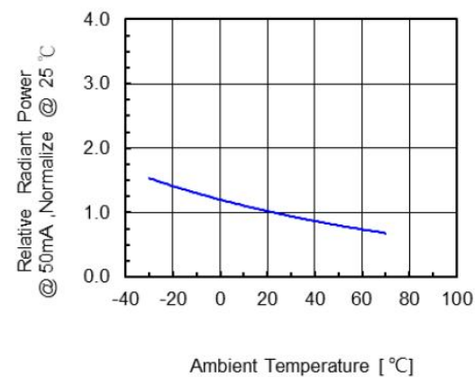
Fig 4. Relative Radiant Power vs. Temperature
