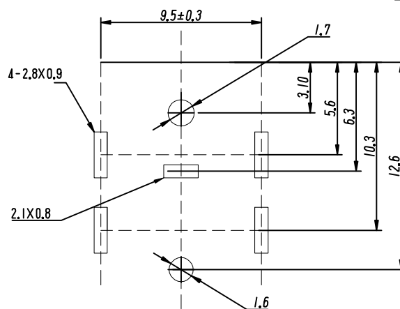
PCB LAYOUT TOP VIEW (TOLERANCE:±0.05)
