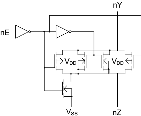
Figure 8-2 Logic diagram (one switch)
