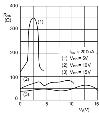
Figure 8-10 Typical R_{ON} as a function of input voltage
