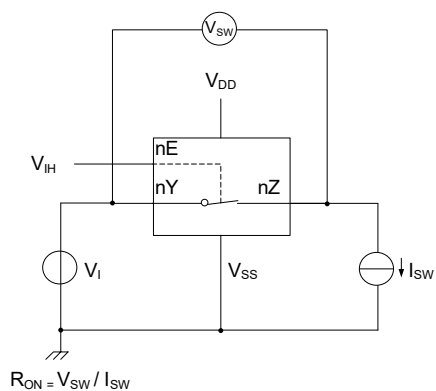
Figure 8-9 Test circuit for measuring R_{ON}
