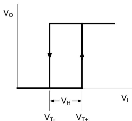
Figure 8-6 Transfer characteristic
