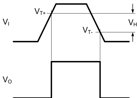
Figure 8-7 Definition of V_{T+} , V_{T-} and V_H
