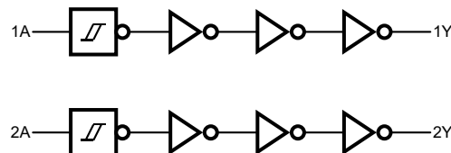
Figure 8-3 Logic diagram
