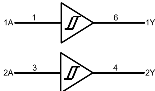
Simplified schematic
