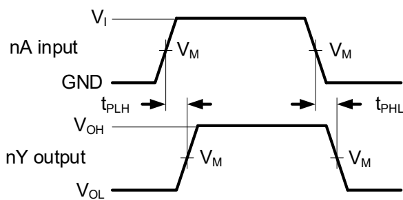
Figure 8-5 The input nA to output nY propagation delays and the output transition times
