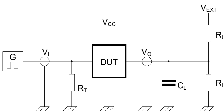
Figure 8-4 Test circuit for measuring switching times
