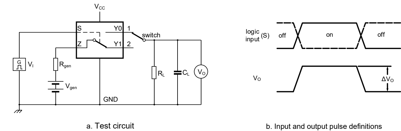
Figure 8-19 Test circuit for measuring charge injection
