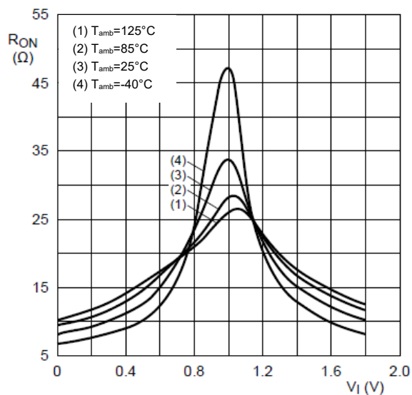
Figure 8-7 ON resistance as a function of input voltage; V_{CC}=1.8V
