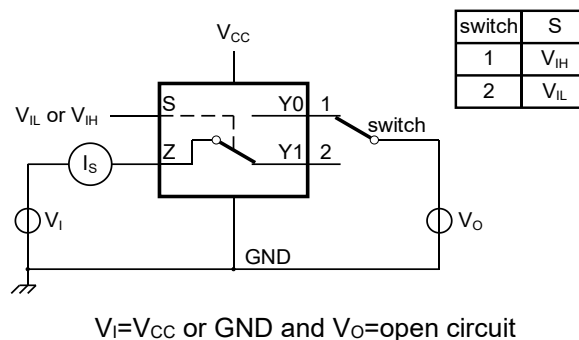
Figure 8-4 Test circuit for measuring ON-state leakage current
