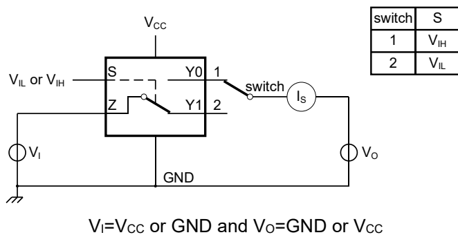
Figure 8-3 Test circuit for measuring OFF-state leakage current
