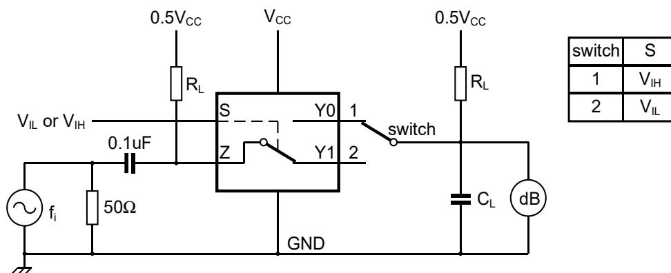
Figure 8-18 Test circuit for measuring isolation (OFF-state)
