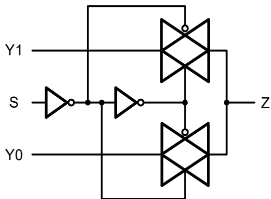
Figure 8-2 Logic diagram
