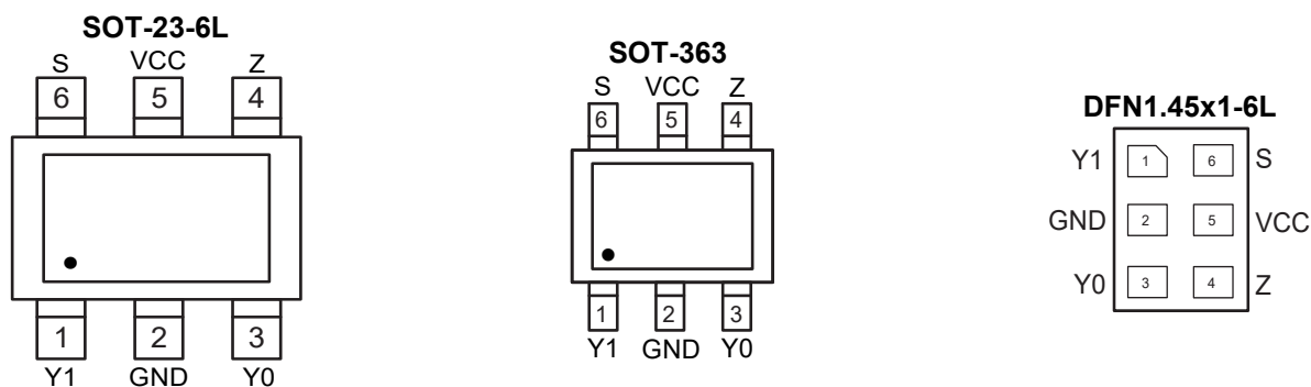
Figure 6-1 Pin configuration
