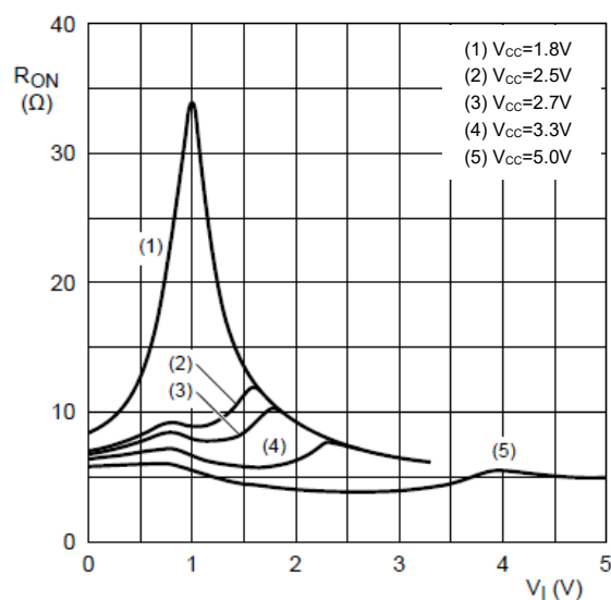
Figure 8-6 Typical ON resistance as a function of input voltage; T_{amb}=25^{\circ}C
