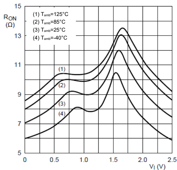
Figure 8-8 ON resistance as a function of input voltage; V_{CC}=2.5V
