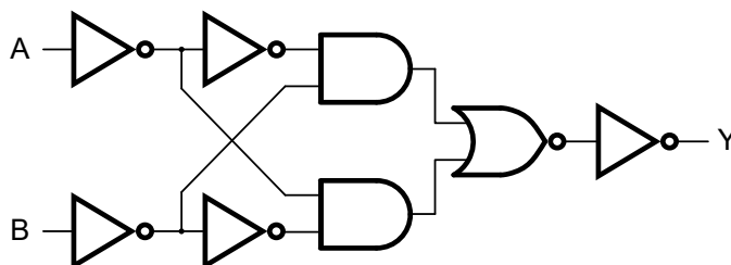
Figure 8-3 Logic diagram for one gate
