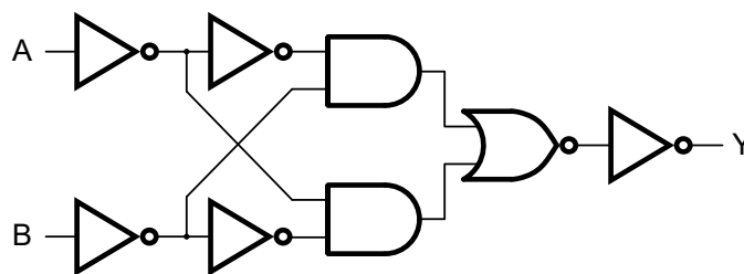
Logic diagram
