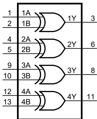
Figure 8-1 Logic symbol
