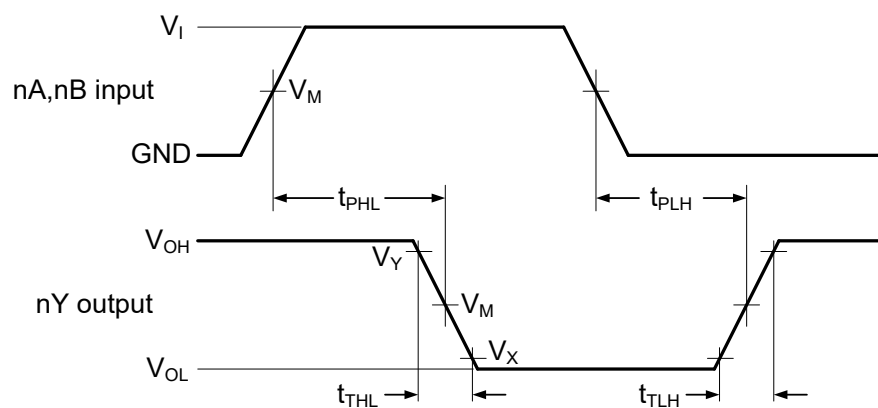
Figure 8-5 Input to output propagation delays
