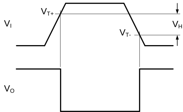
Figure 8-7 Transfer characteristics definitions
