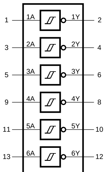
Figure 8-1 Logic symbol
