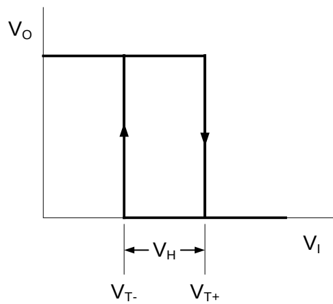
Figure 8-6 Transfer characteristics
