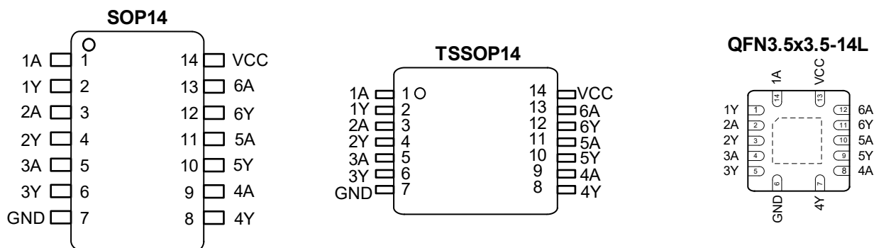
Figure 6-1 Pin configuration
