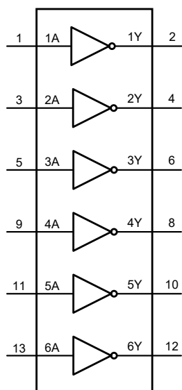
Figure 8-1 Logic symbol
