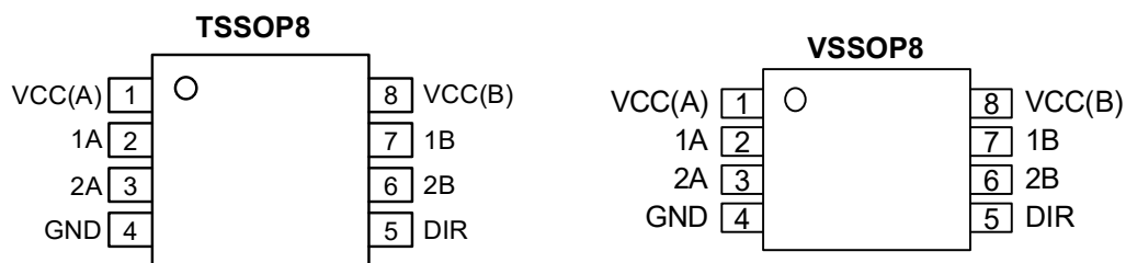
Figure 6-1 Pin configuration
