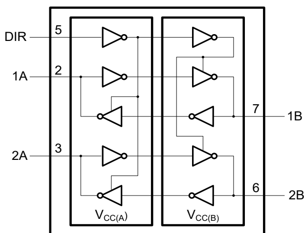
Figure 8-1 Logic symbol
