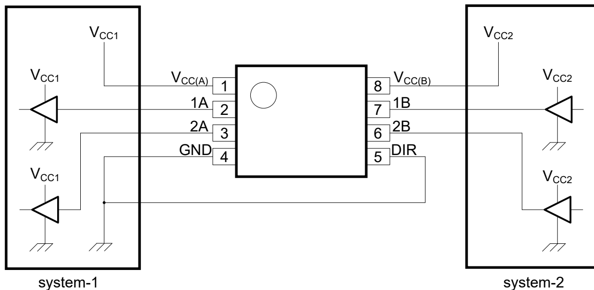
Figure 9-1 Unidirectional logic level-shifting application
