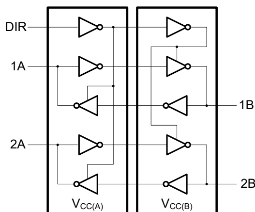
Figure 8-2 Logic diagram
