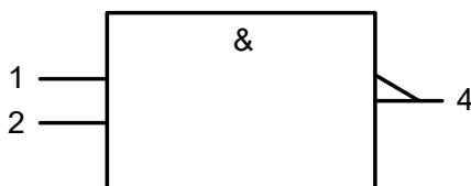
Figure 8-2 IEC logic symbol
