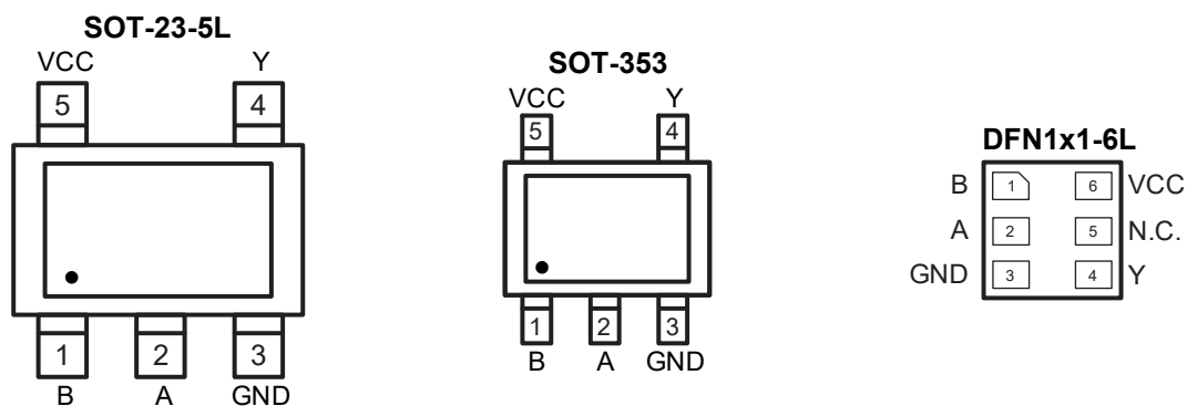
Figure 6-1 Pin configuration
