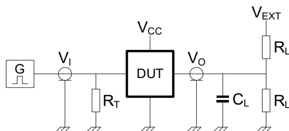
Figure 8-4 Test circuit for measuring switching times
