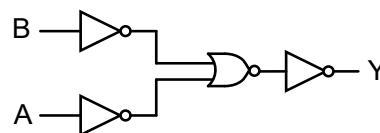
Figure 8-3 Logic diagram
