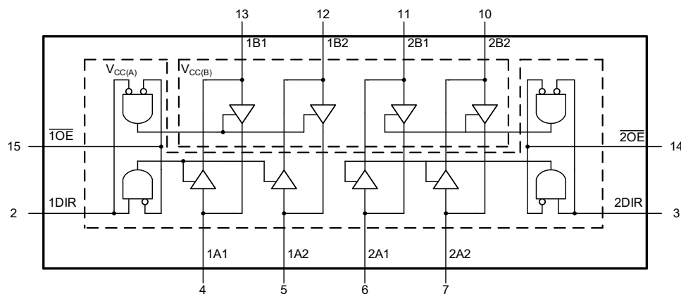
Figure 8-1 Logic symbol
