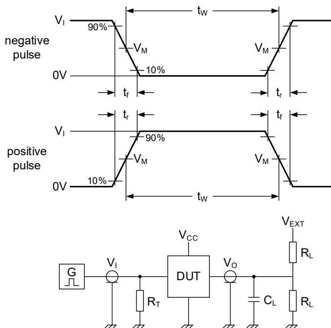
Figure 8-5 Load circuitry for switching times
