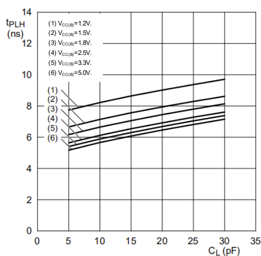
d. LOW to HIGH propagation delay (nBn to nAn)
