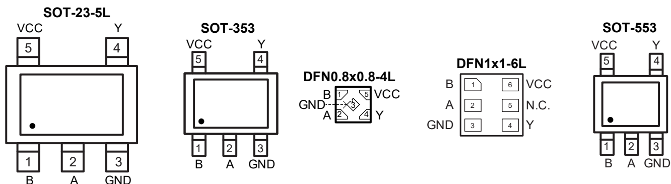
Figure 6-1 Pin configuration
