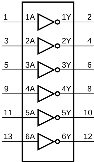
Figure 8-1 Logic symbol
