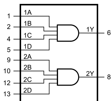
Figure 8-4 Functional diagram
