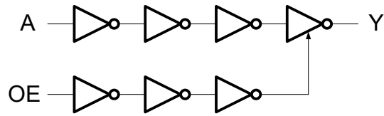
Figure 8-2 Logic diagram
