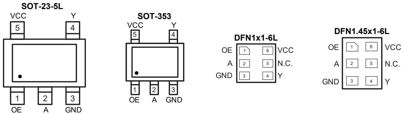
Figure 6-1 Pin configuration
