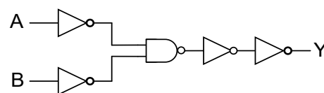
Figure 8-3 Logic diagram
