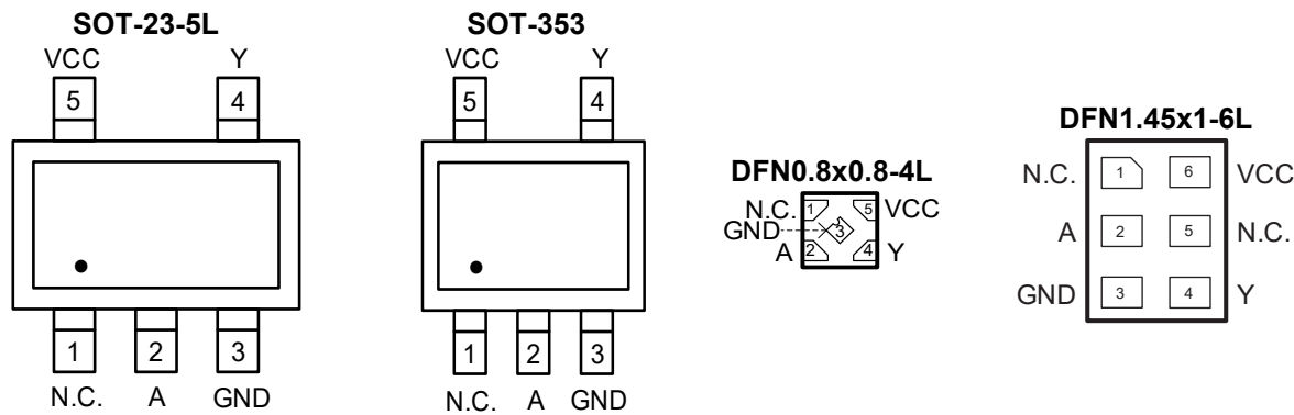
Figure 6-1 Pin configuration
