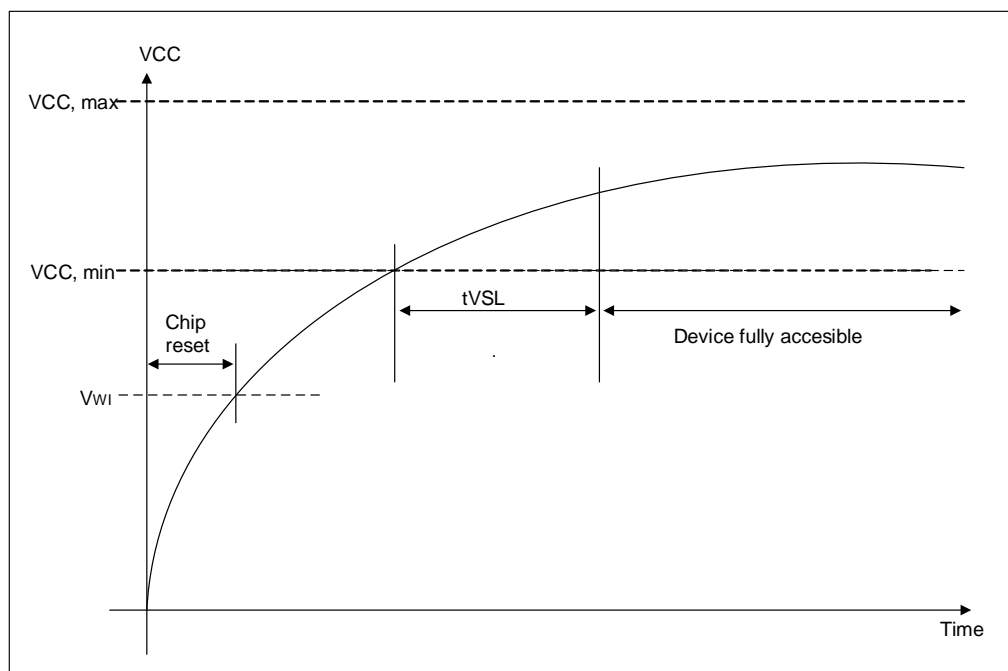
Figure 8.26 Power-Up Timing
