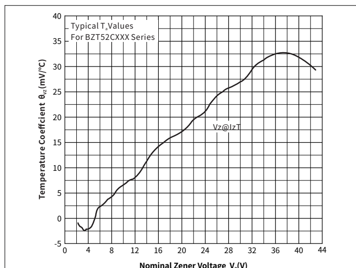
Fig.3 Temperature Coefficients
