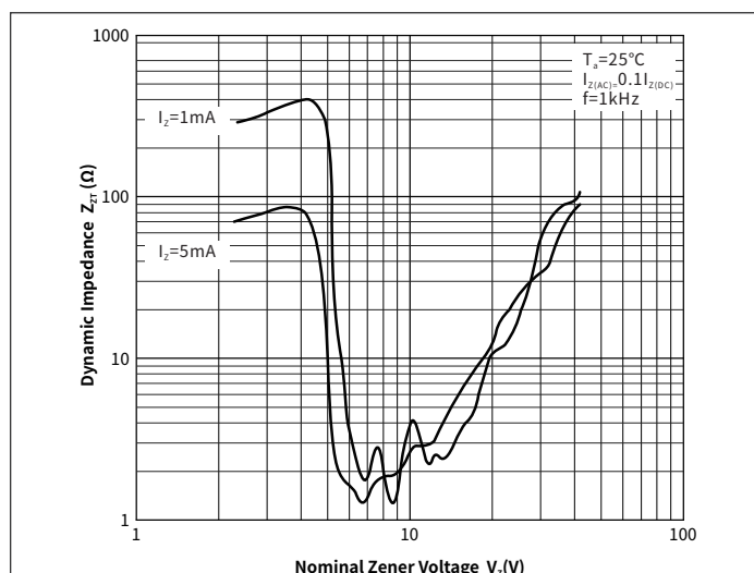
Fig.4 Effect of Zener Voltage on Zener Impedance
