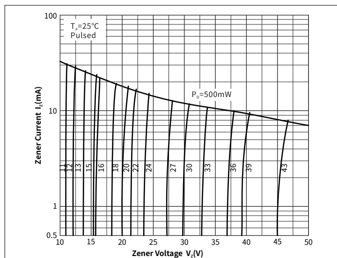
Fig.2 Zener Characteristics(11V to 43V)
