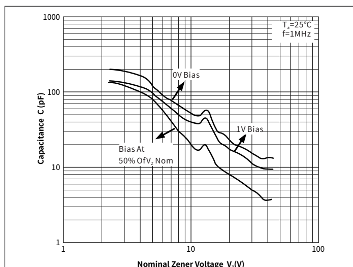
Fig.3 Typical Capacitance
