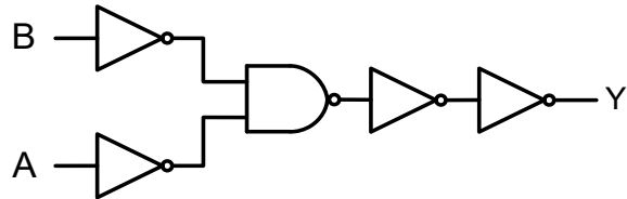
Figure 8-2 IEC logic symbol
