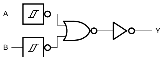
Figure 8-3 Logic diagram for one gate
