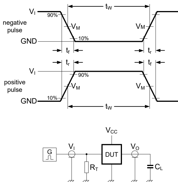
Figure 8-4 Test circuit for measuring switching times
