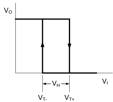
Figure 8-6 Transfer characteristics
