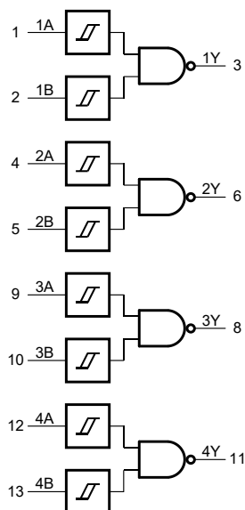
Figure 8-1 Logic symbol
