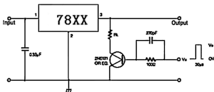
Load Regulation
