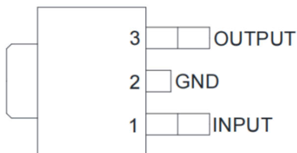
78XX (TO252-2)
