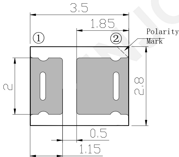
Recommend Pad Layout
