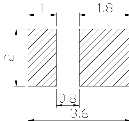
Recommend Pad Layout
