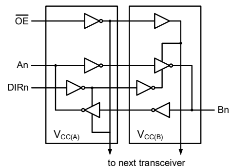
Logic diagram
