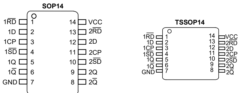
Figure 6-1 Pin configuration
