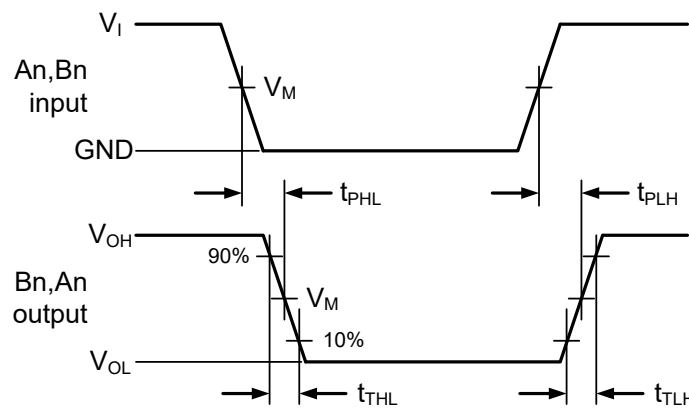
Figure 8-3 The data input (An, Bn) to data output (Bn, An) propagation delay times
