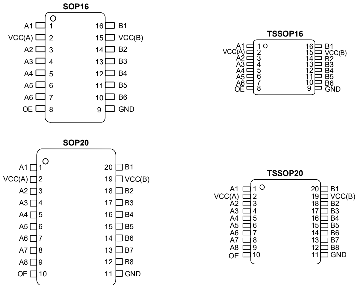
Figure 6-1 Pin configuration
