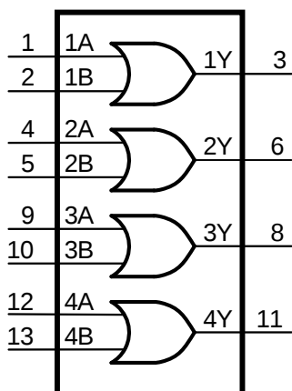
Figure 8-1 Logic symbol
