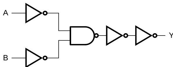
Figure 8-3 Logic diagram for one gate
