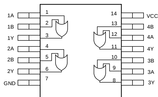
Functional pinout
