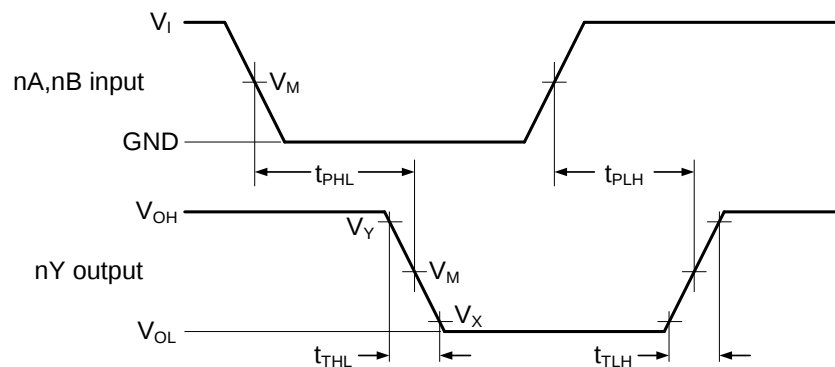
Figure 8-5 Input to output propagation delays
