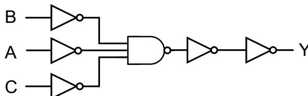
Figure 8-1 Logic symbol
