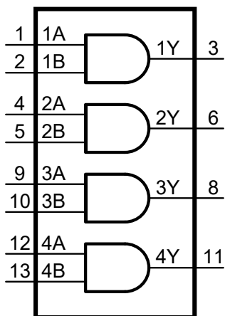
Figure 8-1 Logic symbol
