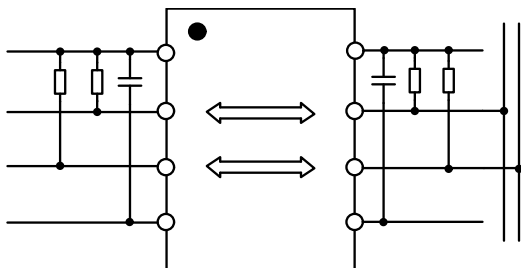
Figure 22. Typical Isolated I 2 C Interface Using the SI8400AB-A-IS
