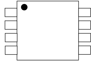
Figure 3. Pin Configuration
