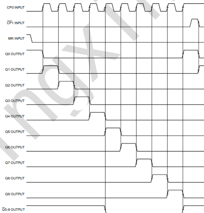
Figure 5. Timing diagram
