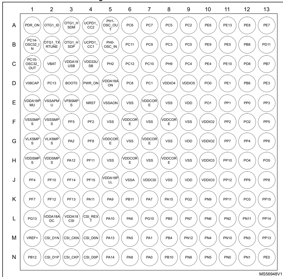
Figure 9. VFBGA169GP ballout
