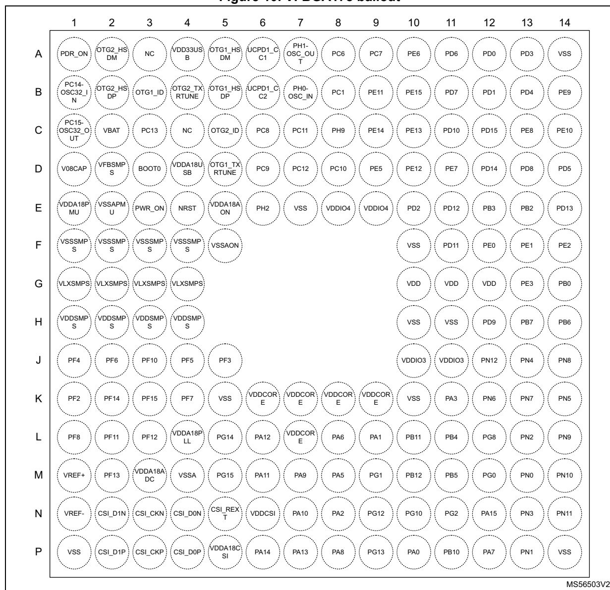
Figure 10. VFBGA178 ballout
