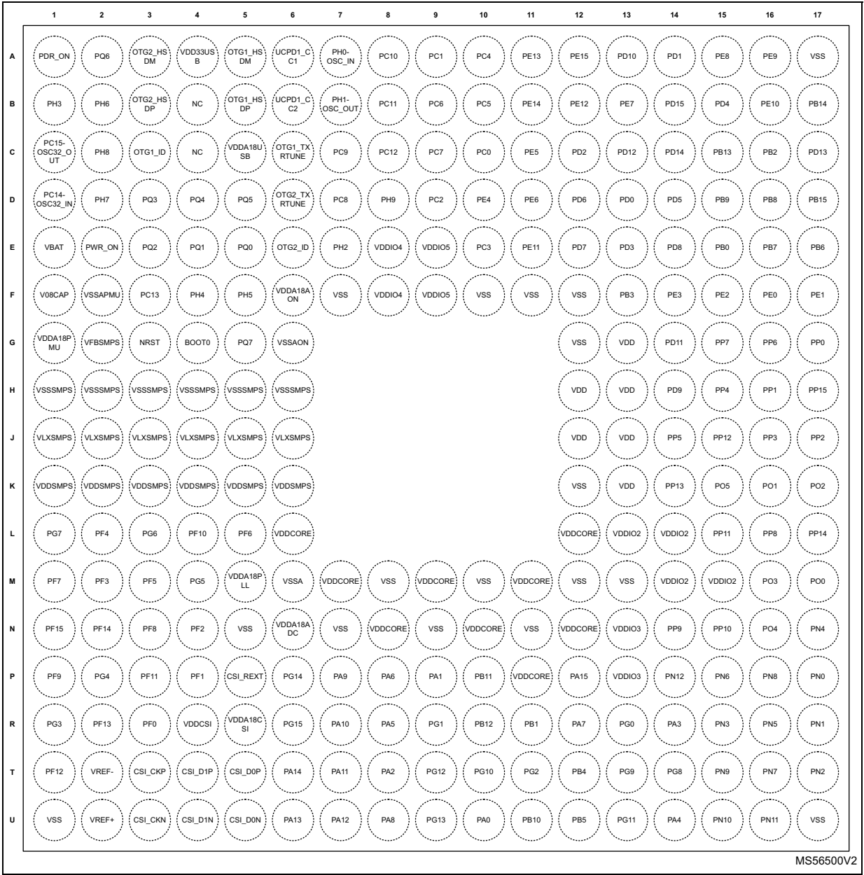
Figure 13. VFBGA264 ballout
