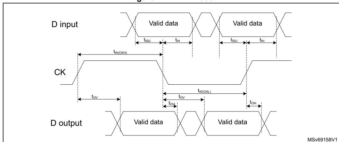
Figure 44. DDR mode
