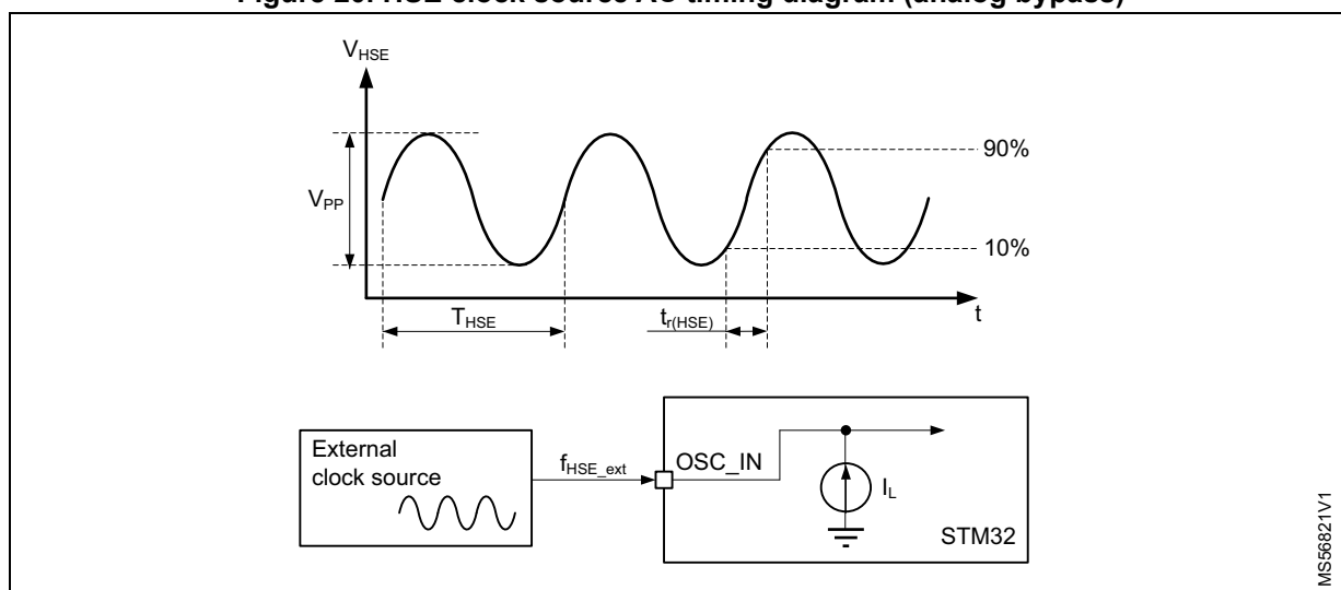
Figure 20. HSE clock source AC timing diagram (analog bypass)
