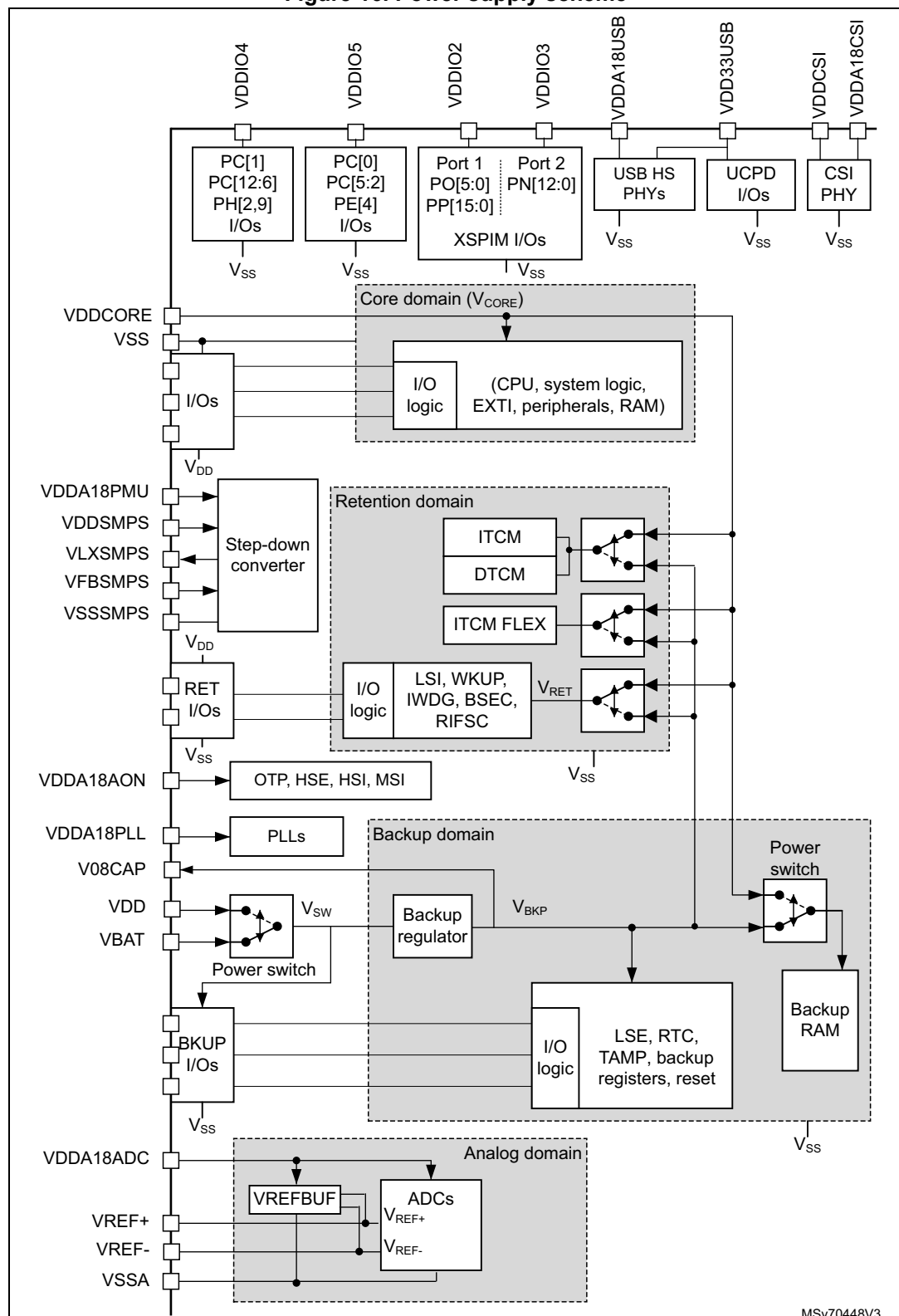
Figure 16. Power supply scheme
