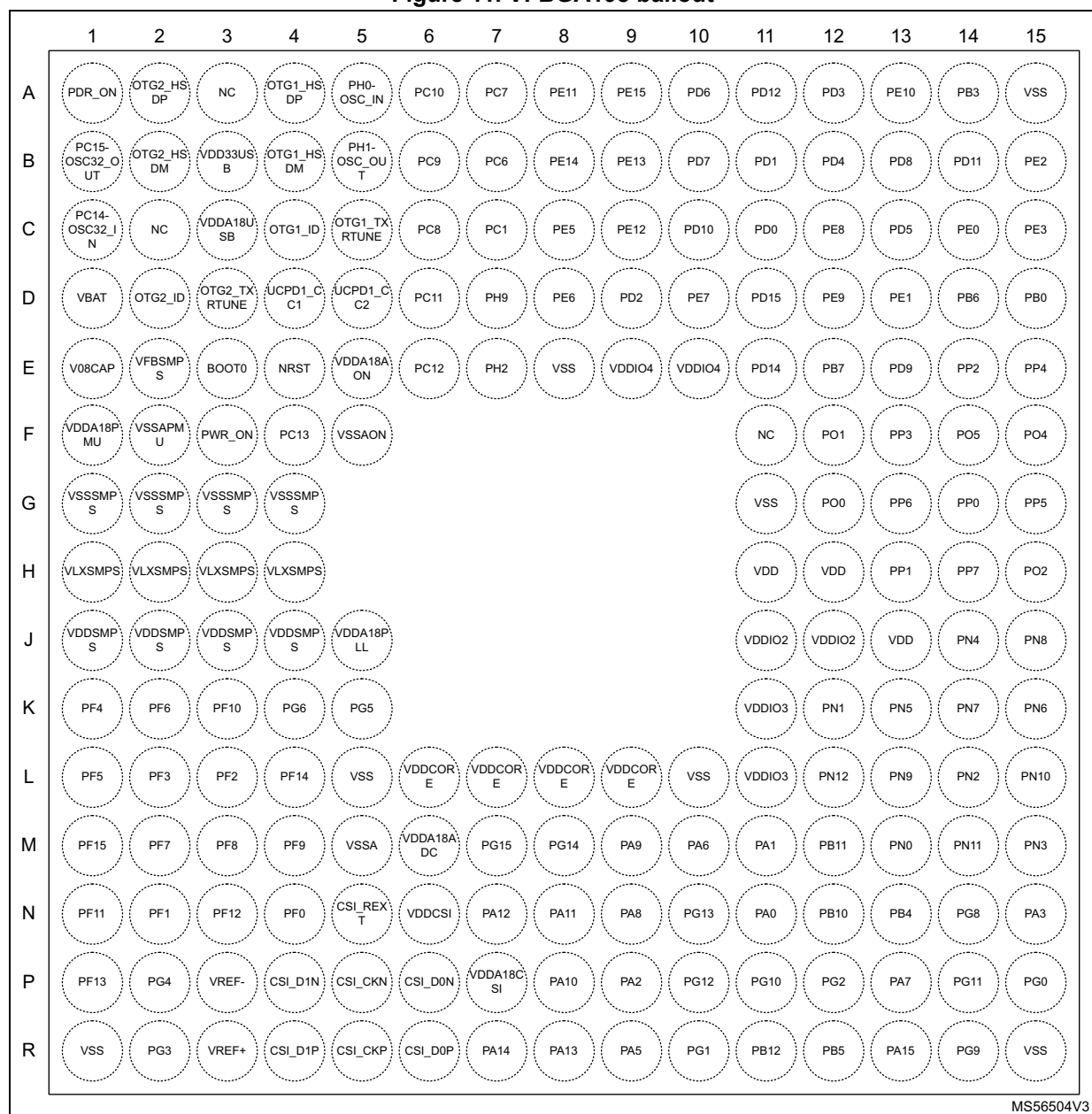
Figure 11. VFBGA198 ballout
