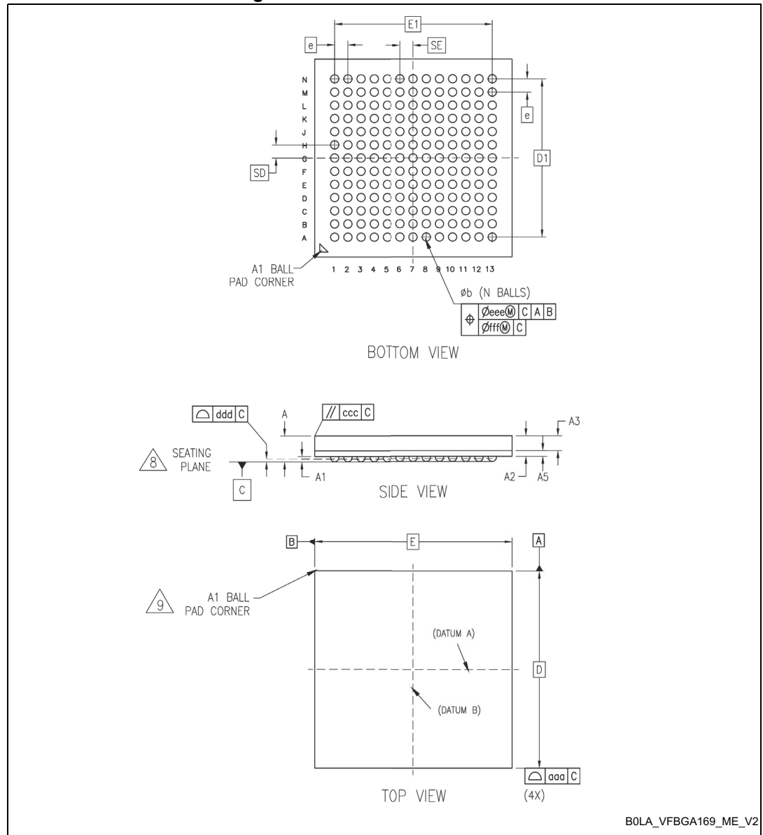
Figure 68. VFBGA169 - Outline (13)
