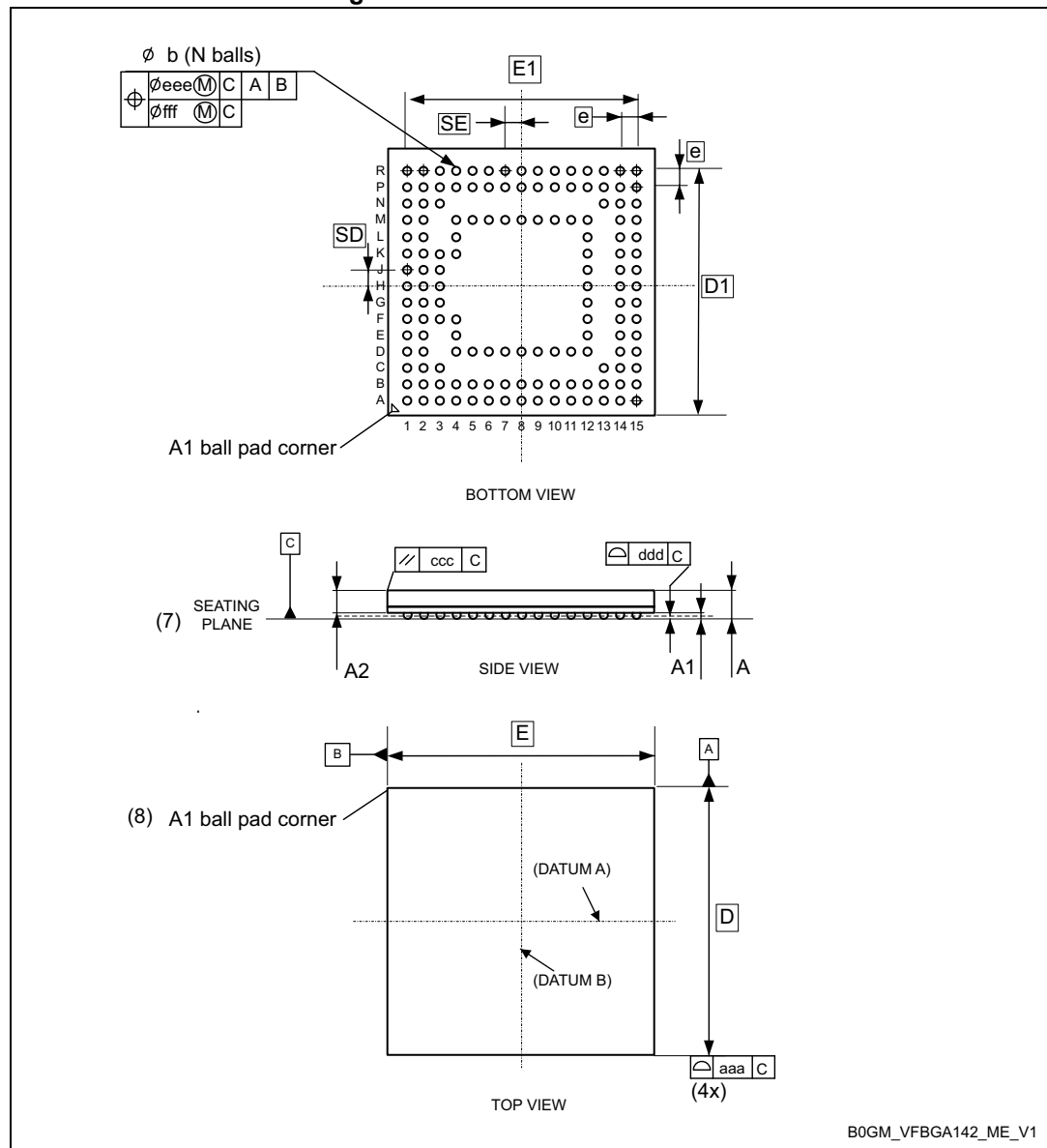
Figure 67. VFBGA142 - Outline (13)
