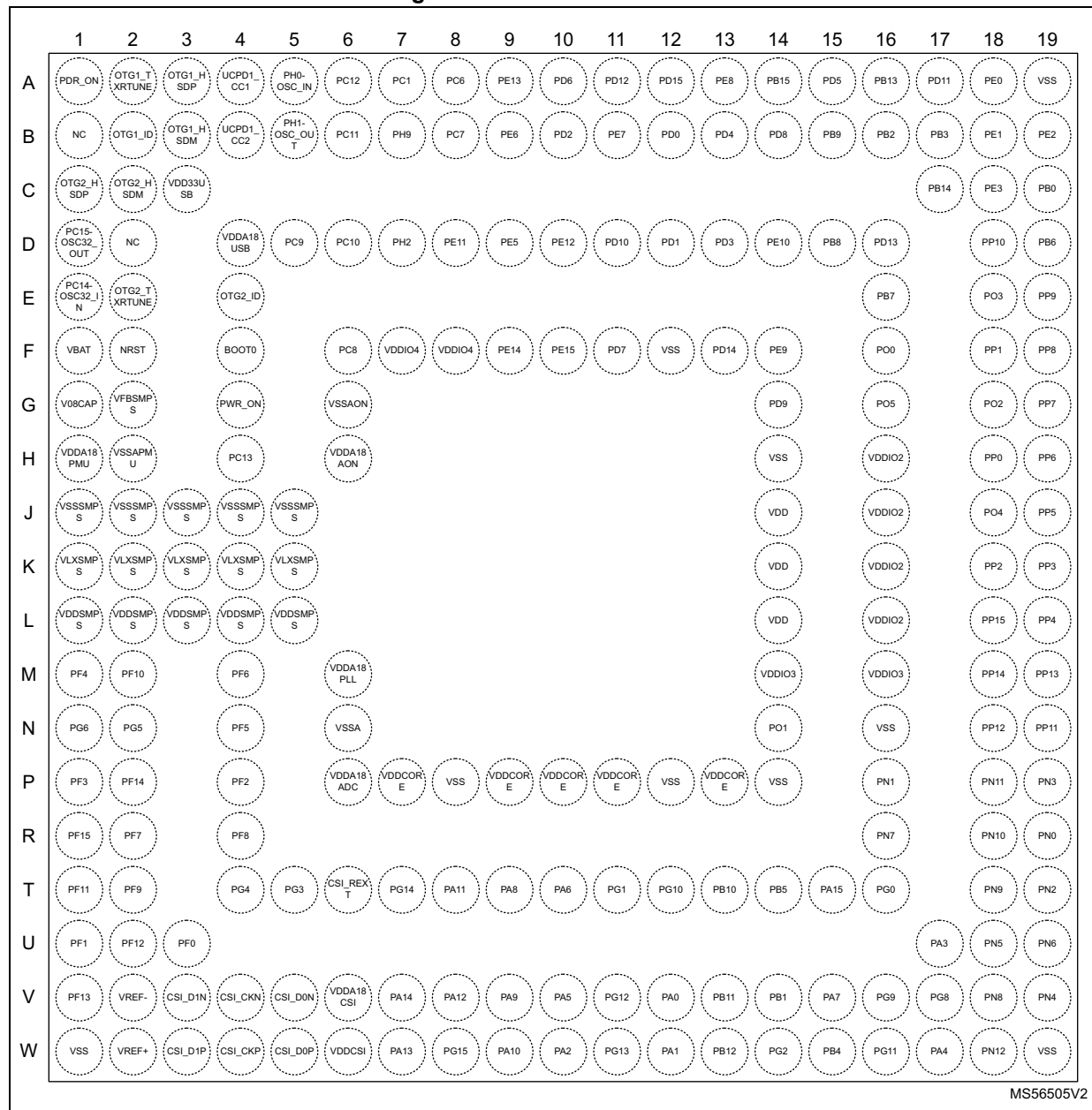
Figure 12. VFBGA223 ballout
