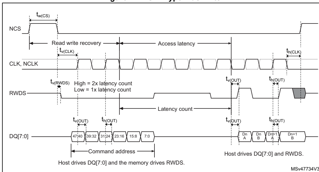
Figure 41. XSPI HyperBus write
