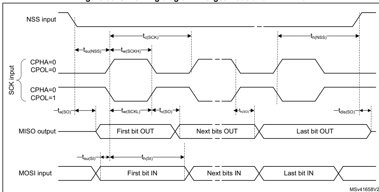
Figure 56. SPI timing diagram - Target mode and CPHA = 0
