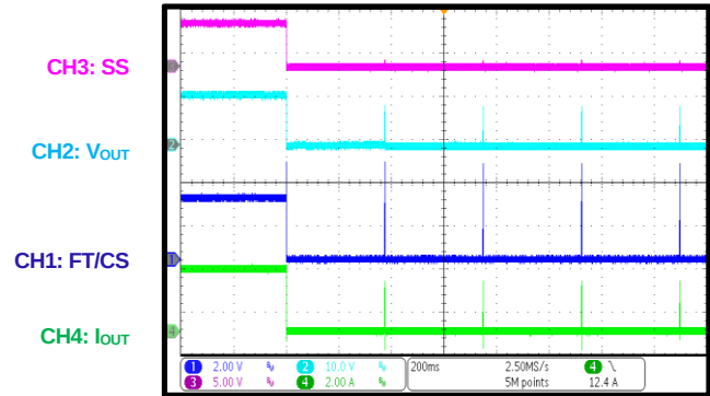
Load Dump
