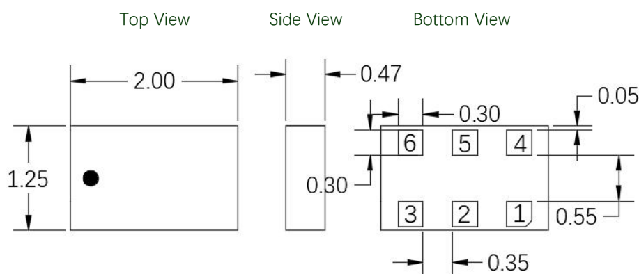
Figure 2. MHC25S03 Outline Drawing
