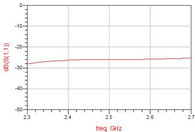
Figure 5. MHC25S03 Return Loss (S11)
