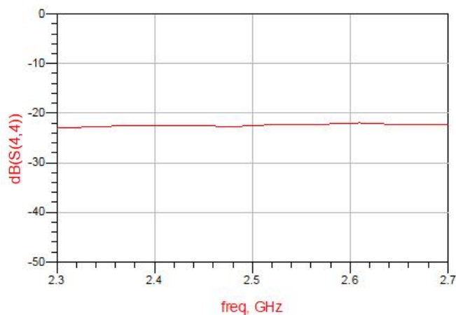
Figure 7. MHC25S03 Return Loss (S44)
