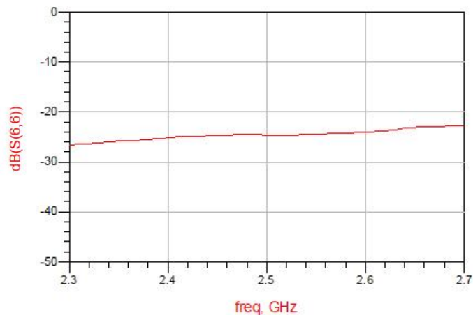
Figure 8. MHC25S03 Return Loss (S66)
