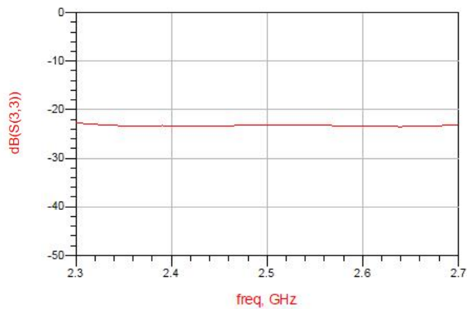
Figure 6. MHC25S03 Return Loss (S33)
