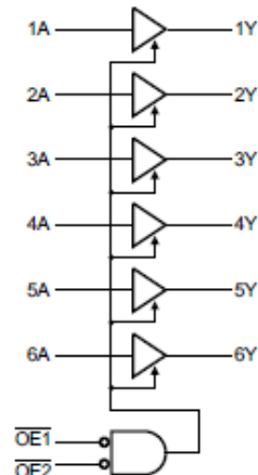
Figure 1. Logic symbol
