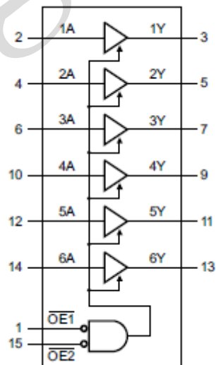
Figure 3. Functional diagram
