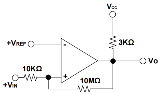
Non-Inverting Comparator with Hysteresis
