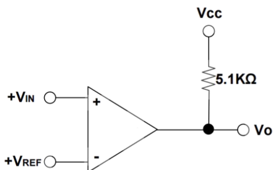
Basic Comparator
