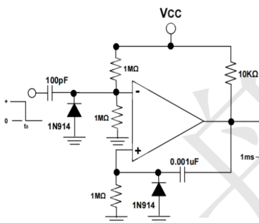
One-Shot Multivibrator
