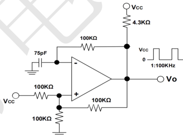
Squarewave Oscillator
