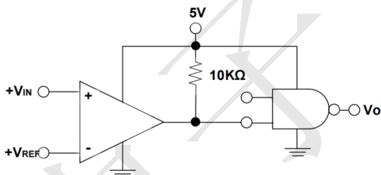
Driving CMOS/TTL
