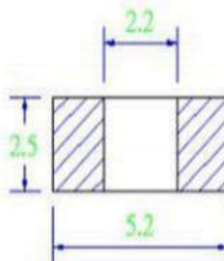
Recommend Land Pattern Dimensions
