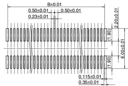
Recommended metal mask pattern Metal mask thickness: When 120 \mu m (Opening area ratio: 87%)
