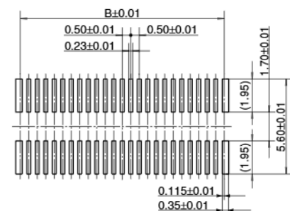
Recommended metal mask pattern Metal mask thickness: When 120 \mu m (Opening area ratio: 78%)
