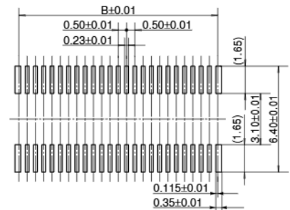
Recommended metal mask pattern Metal mask thickness: When 120 \mu m (Opening area ratio: 76%)
