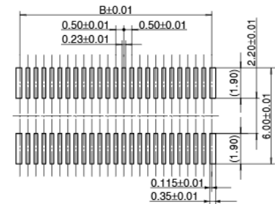
Recommended metal mask pattern Metal mask thickness: When 120 \mu m (Opening area ratio: 87%)
