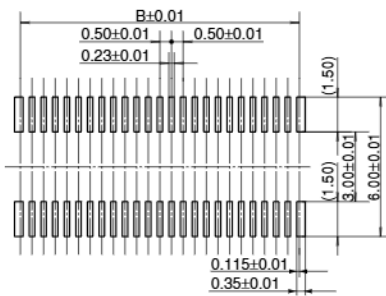
Recommended metal mask pattern Metal mask thickness: When 150 \mu m (Opening area ratio: 69%)
