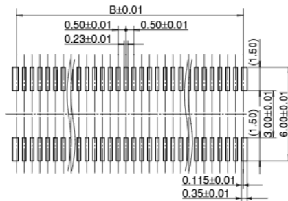
Recommended metal mask pattern Metal mask thickness: When 150 \mu m (Opening area ratio: 60%)
