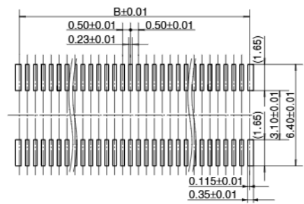
Recommended metal mask pattern Metal mask thickness: When 120 \mu m (Opening area ratio: 76%)
