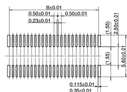
Recommended metal mask pattern Metal mask thickness: When 150 \mu m (Opening area ratio: 62%)
