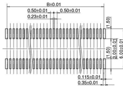
Recommended metal mask pattern Metal mask thickness: When 150 \mu m (Opening area ratio: 69%)
