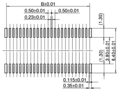
Recommended metal mask pattern Metal mask thickness: When 150 \mu m (Opening area ratio: 60%)
