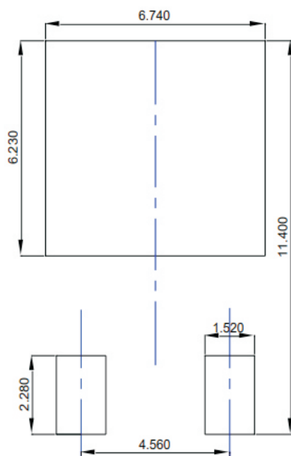
SUGGESTED SOLDER PAD LAYOUT
