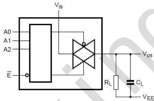
Figure 10. Crosstalk logical input/output test
