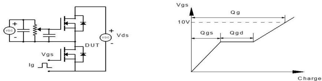
Figure 1: Gate Charge Test Circuit & Waveform
