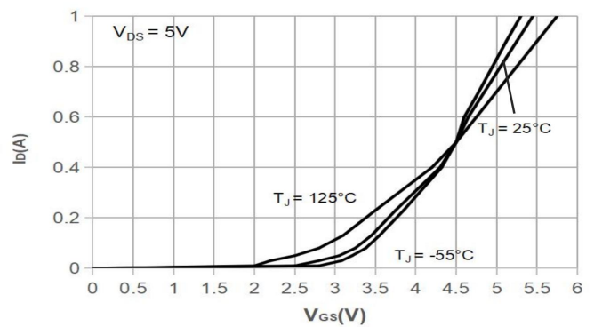
Figure 2: Typical Transfer Characteristics
