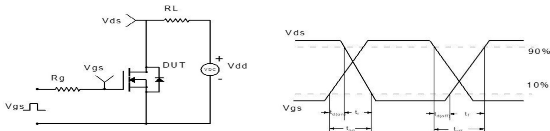
Figure 2: Resistive Switching Test Circuit & Waveform
