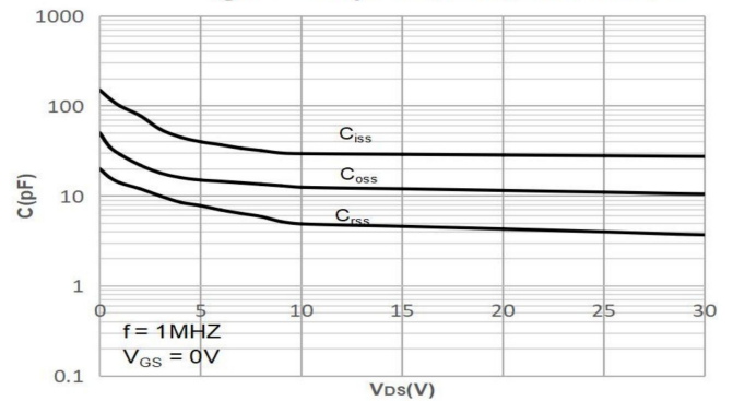
Figure 6: Capacitance Characteristics
