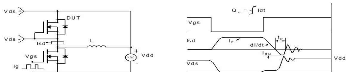
Figure 4: Diode Recovery Test Circuit & Waveform
