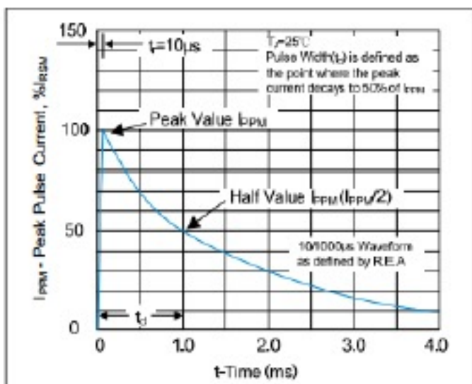
Figure 3. Pulse Waveform
