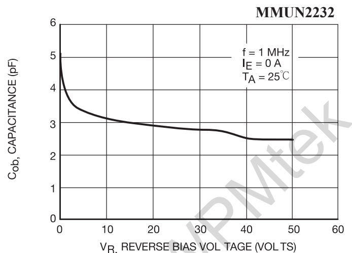
Figure 24. Output Capacitance
