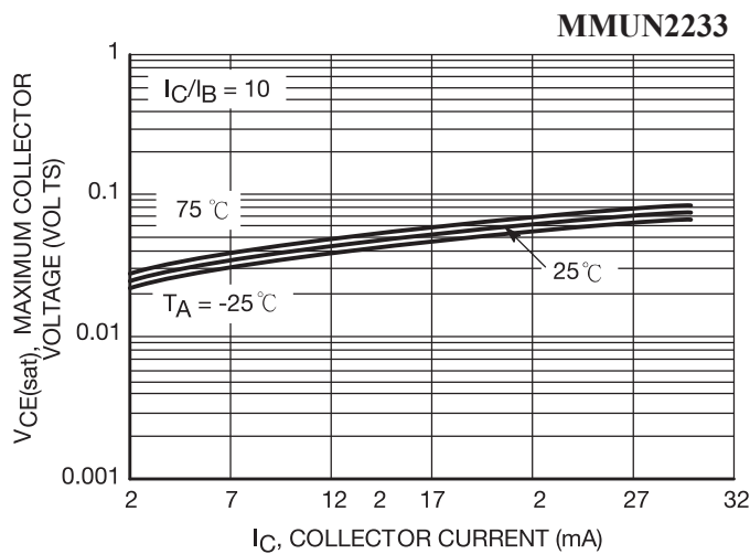
Figure 27. V_{CE(sat)} vs. I_C
