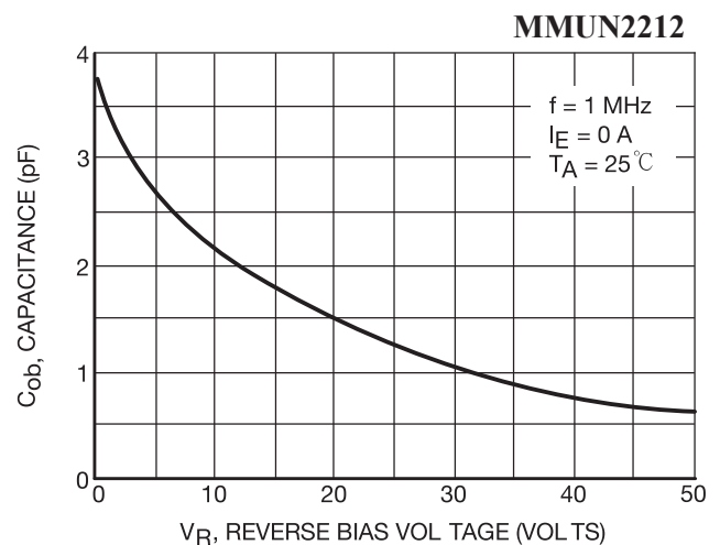
Figure 4. Output Capacitance
