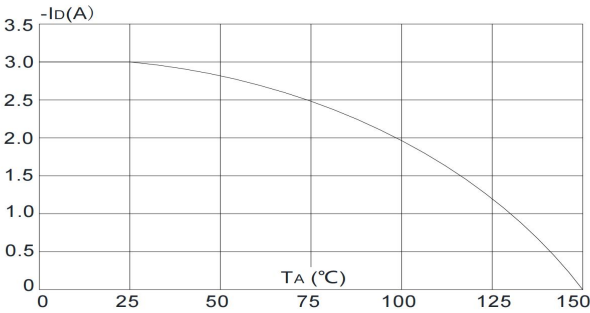
Figure 10: Maximum Continuous Drain Current vs. Ambient Temperature
