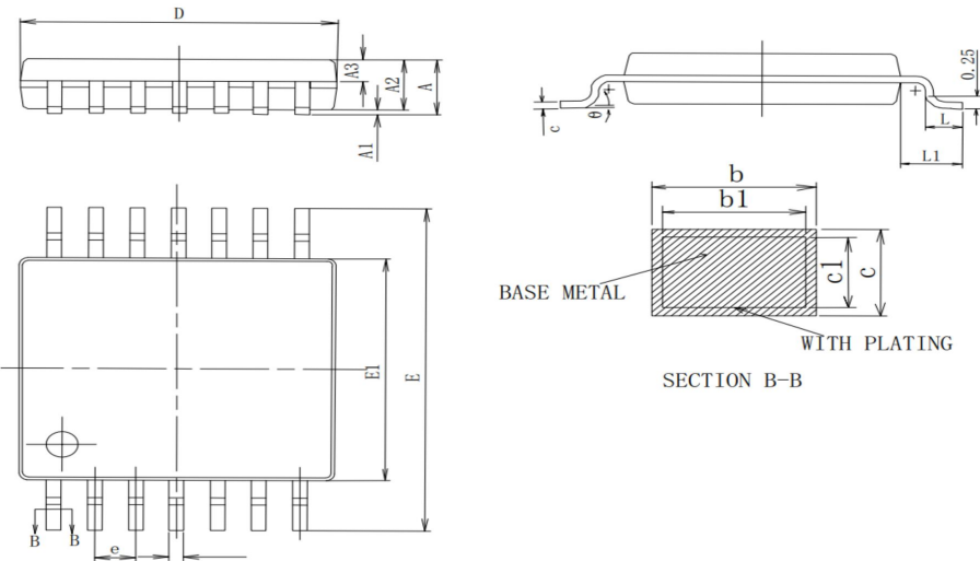
TSSOP 14 package information
