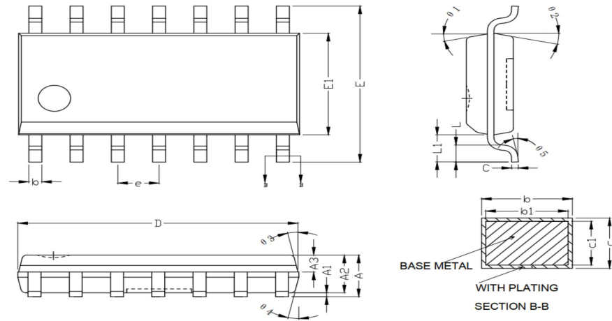
SOP 14 package information
