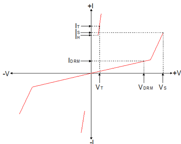
V-I Curve
