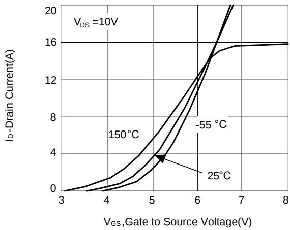
Figure 1: Transfer Characteristics
