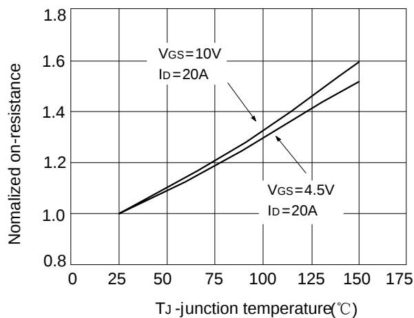
Fig.2 rdson-junction temperature
