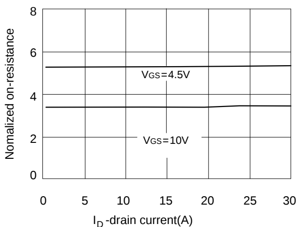
Fig.5 rdson-drain current
