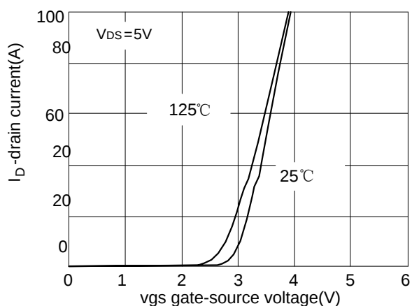
Fig.3 transfer characteristics
