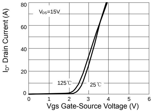
V GS Gate-Source Voltage (V) Figure 3: Transfer characteristics
