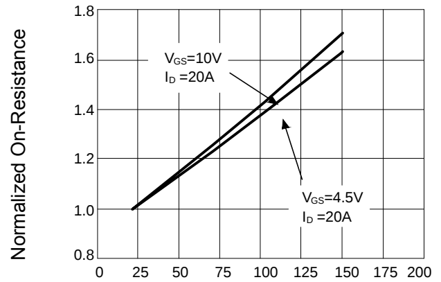
T J -Junction Temperature(°C) Figure 2: Rdson-junction temperature
