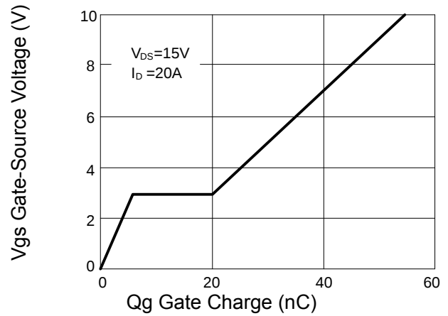
Figure 5: Gate charge
