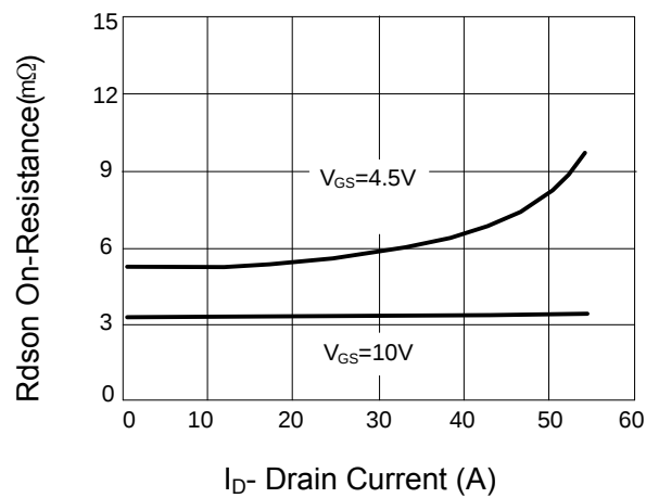
Figure 5: Rdson-drain current
